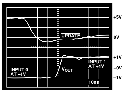
TPC 27. AD8114 Switching Time
