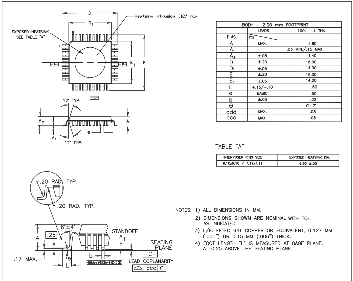
Figure 10. Package 100 pin TQFP. All dimensions are in mm.
