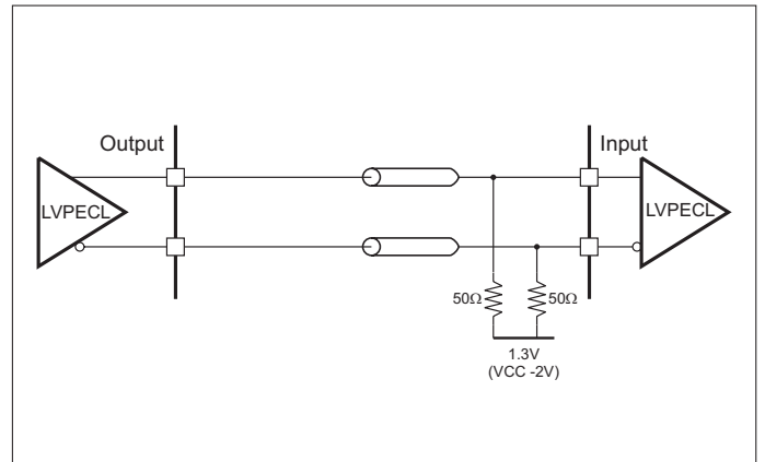
Figure 4. DC Coupled Clock Outputs
