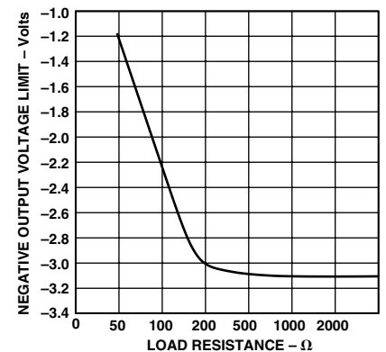
Figure 24. Typical Output Voltage Swing vs. Load Resistance (Negative Output Swing Limits First)
