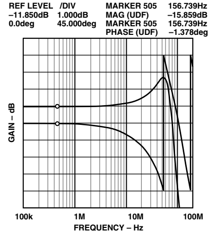
Figure 18. Frequency and Phase Response vs. Gain (Gain = +10 dB, P_{IN} = -30 dBm, Pin 5 Connected to Pin 7)
